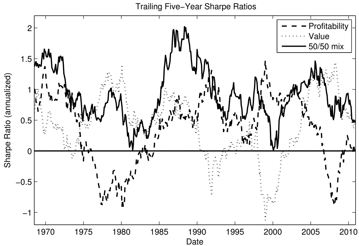
Fig. 1. Performance over time of profitability and value strategies
